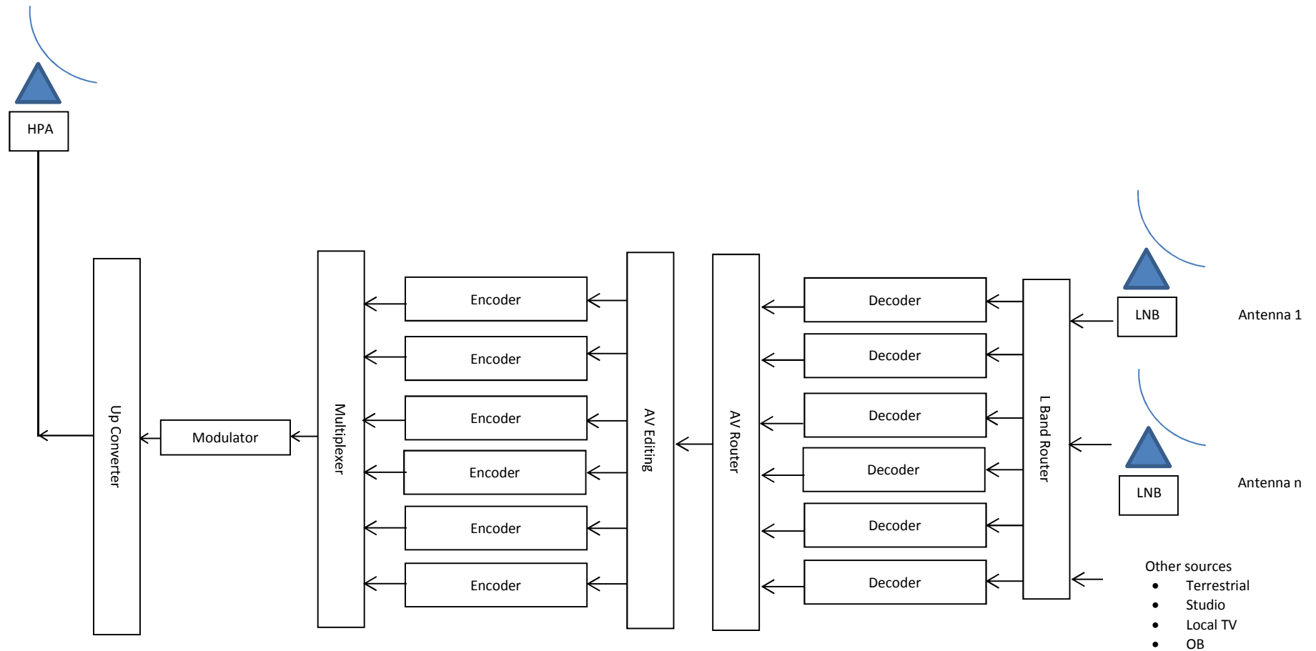
Block Diagram – Digital Turnaround System
