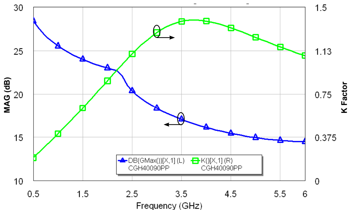
Maximum Available Gain and K Factor of the CGH40090PP
