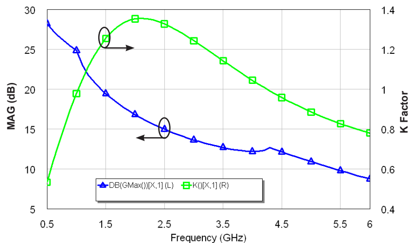
Simulated Maximum Available Gain and K Factor of the CGH40120
