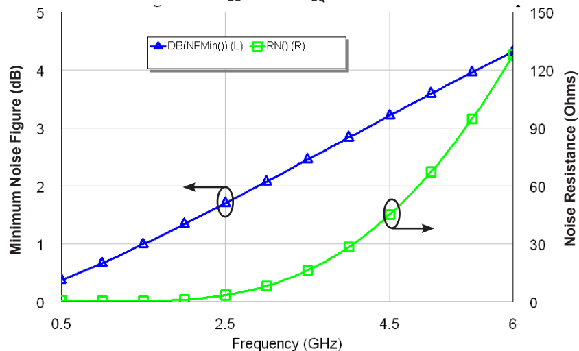
Simulated Minimum Noise Figure and Noise Resistance vs Frequency of the CGH40120
