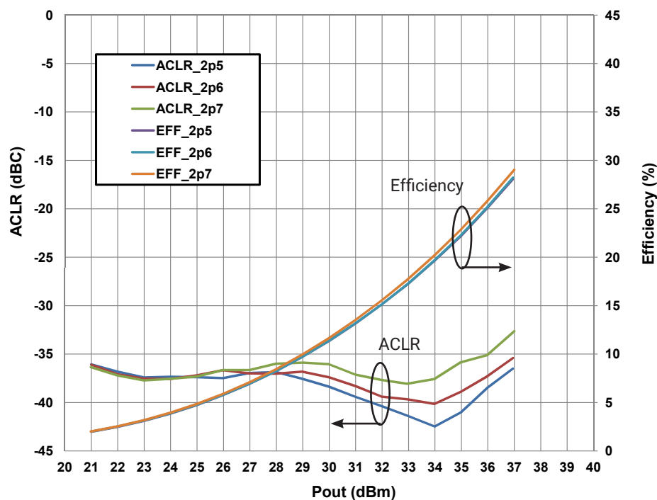
Figure 2. - Typical Drain Efficiency and ACLR vs. Output Power V_{DD} = 50\text{ V} , I_{DQ} = 0.13\text{ A} , 1c WCDMA, PAR = 7.5 dB
