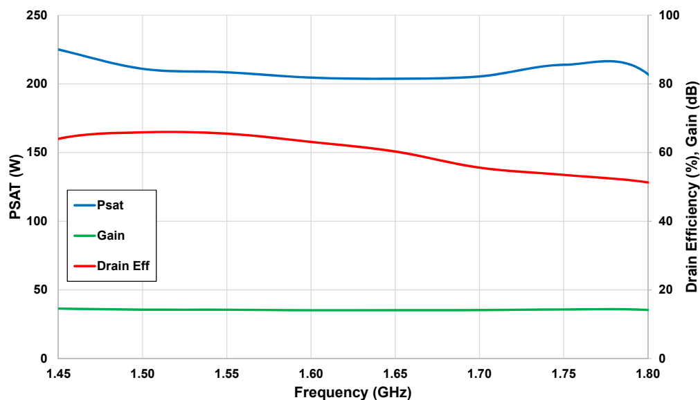
Figure 6. - Saturated Output Power Gain, and Drain Efficiency vs Frequency of the CGHV40200PP measured in the CGHV40200PP Broadband Amplifier Circuit
