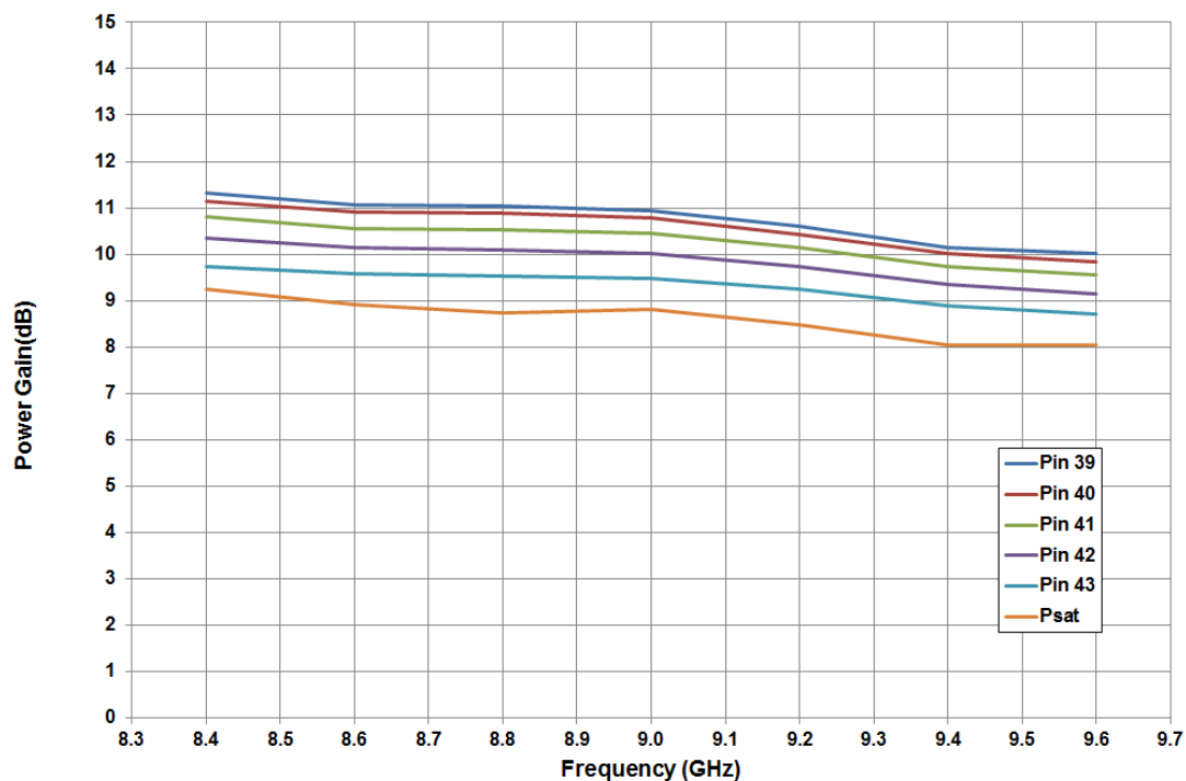
Figure 2. - Power Gain vs. Frequency and Input Power
