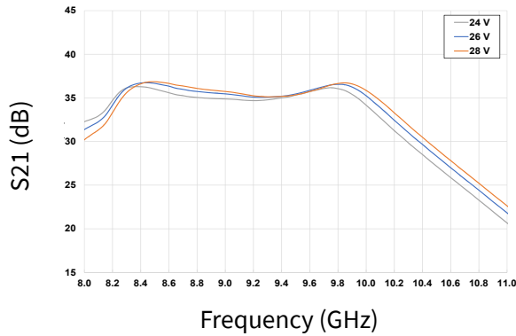
Figure 34. Gain vs Frequency as a Function of Voltage
