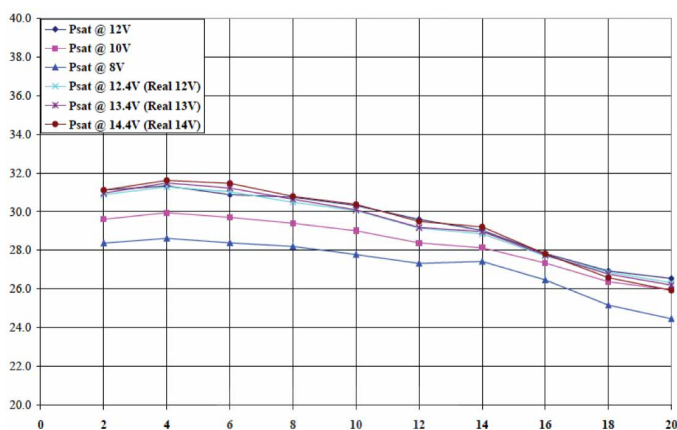
Psat Data (dBm)
