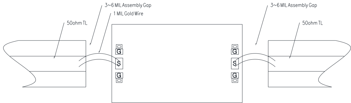
Assembly Diagram
