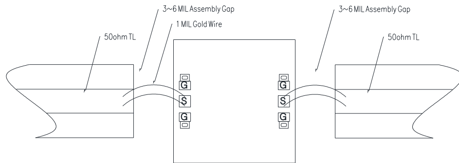
Assembly Diagram
