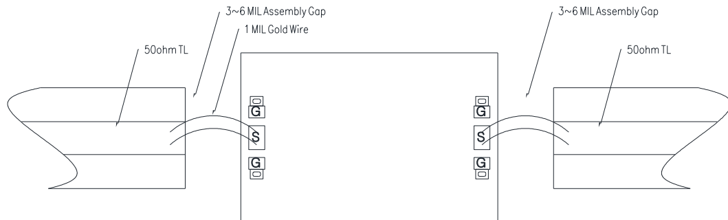
Assembly Diagram
